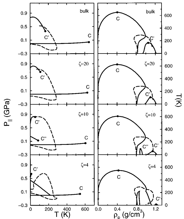
FIG. 10. Phase diagrams for the associating fluid film as determined by the second level of approximation (i.e., with the inhomogeneous reference fluid) in the P_{||} - T (left) and T - \rho_p (right) planes. From bottom to top, the phase behaviors correspond to pores of dimensionless width \zeta=4, 10, 20 , and \infty , respectively. Solid lines represent loci of phase coexistence and the dashed lines are TMDs (states with \alpha_{||}=0 ). The liquid-vapor ( C ) and the liquid-liquid ( C' ) critical points are also shown. Notice that a third fluid-fluid phase transition that terminates in a critical point ( C'' ) appears for dimensionless pore width \zeta=10 .
